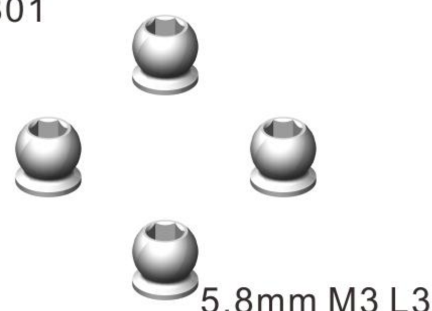
BALL UNIVERSAL 5.8mm M3 L3 HEX H3.0
