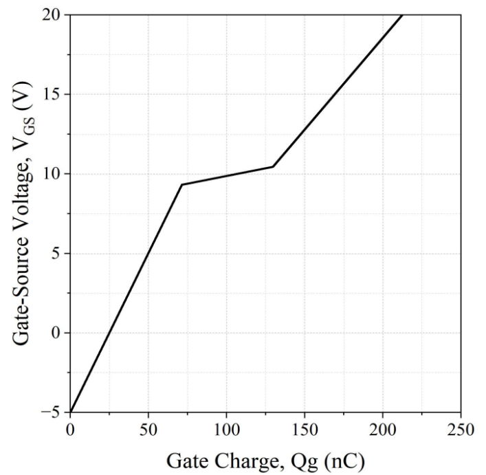
Fig 10. Gate Charge Characteristics
