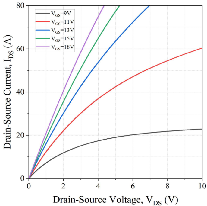
Fig 1. Output Characteristics at T_j = 25^\circ\text{C}
