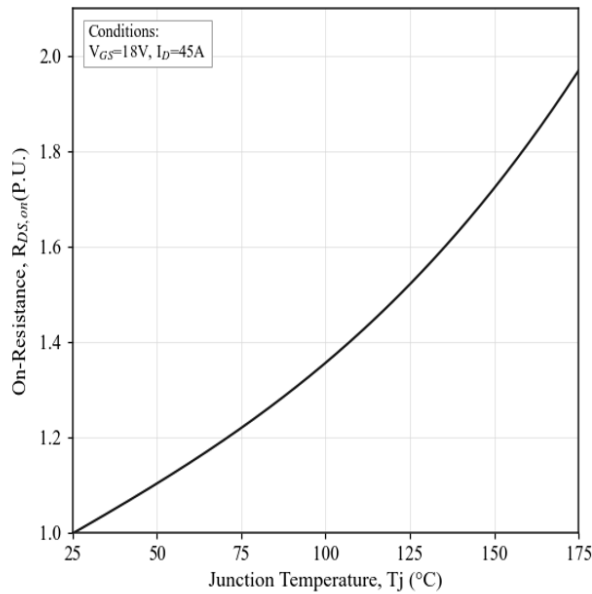
Fig 7. Normalized On-Resistance vs. Temperature
