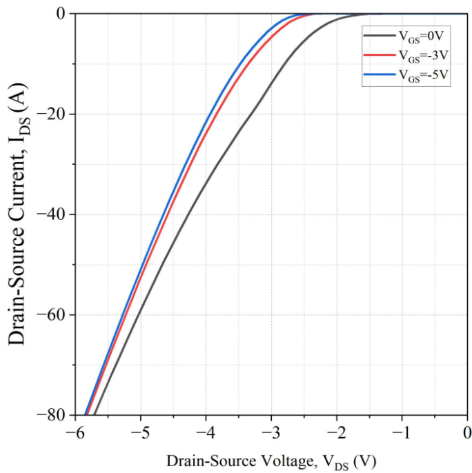
Fig 13. Body Diode Characteristics at Tj= 25°C
