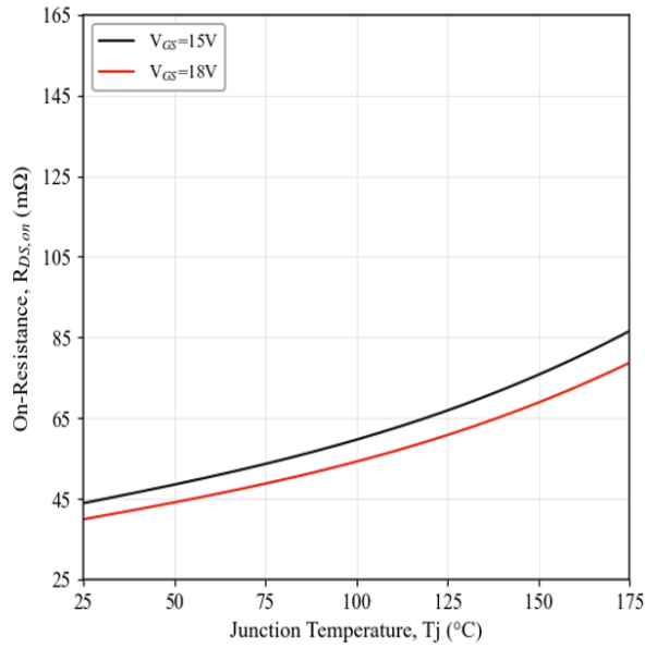
Fig 5. On-Resistance vs. Temperature
