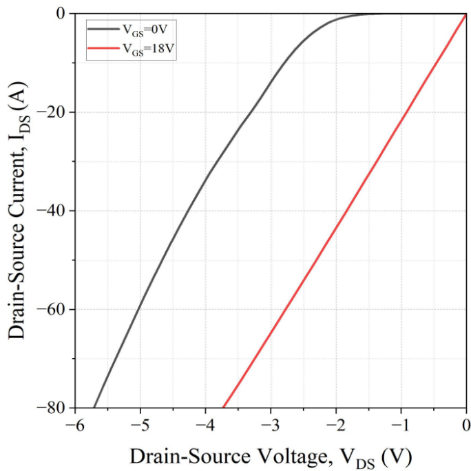
Fig 15. 3rd Quadrant Characteristic at Tj= 25°C
