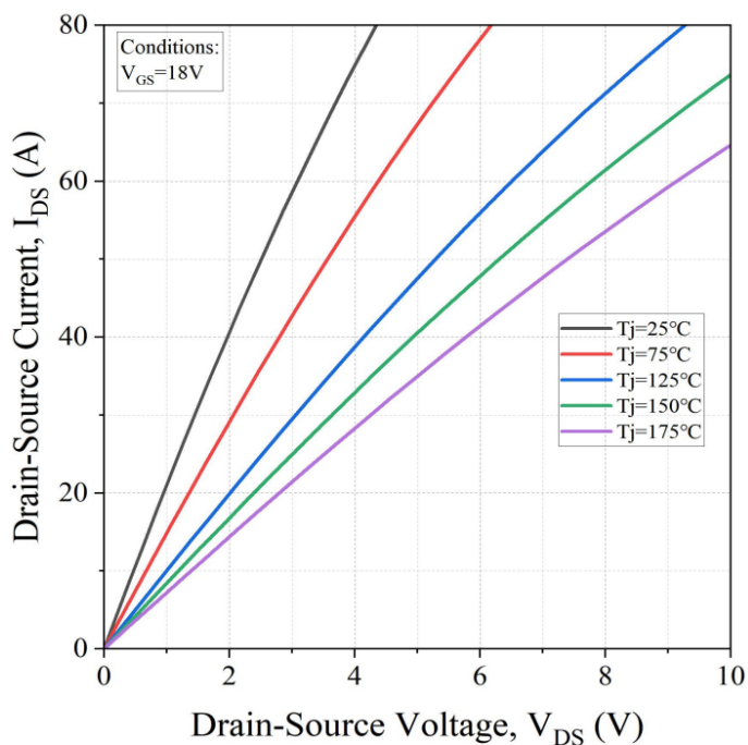
Fig 3. Output Characteristics vs. Temperature
