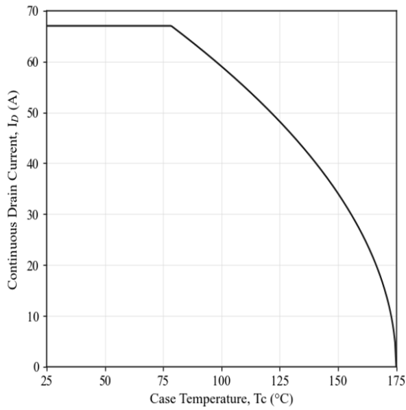
Fig 17. Current De-rating
