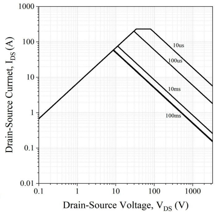
Fig 20. Safe Operating Area
