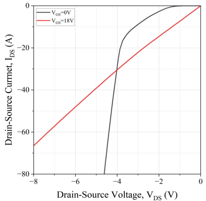
Fig 16. 3rd Quadrant Characteristic at Tj= 175°C
