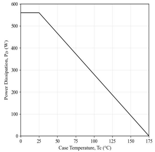
Fig 18. Power Dissipation De-rating
