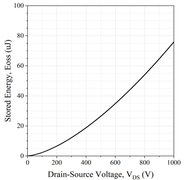
Fig 12. Output Capacitor Stored Energy
