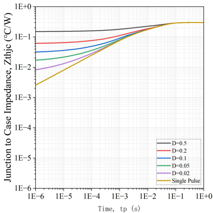
Fig 19. Transient Thermal Impedance
