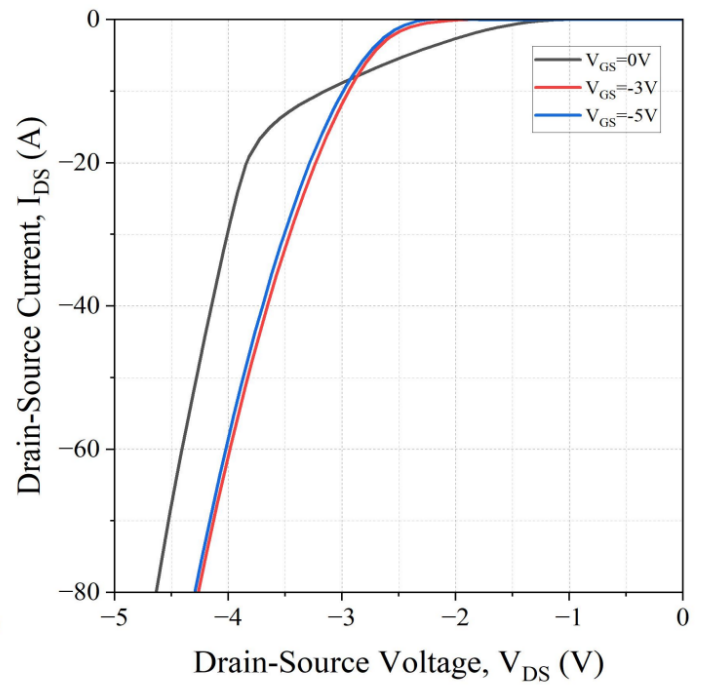
Fig 14. Body Diode Characteristics at Tj= 175°C
