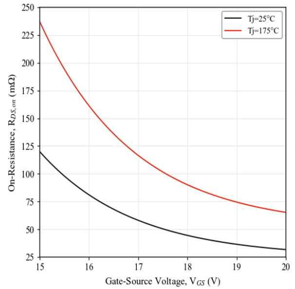
Fig 8. On-Resistance vs. Gate Voltage
