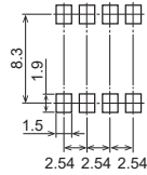
Recommended mounting pad (Top view)
