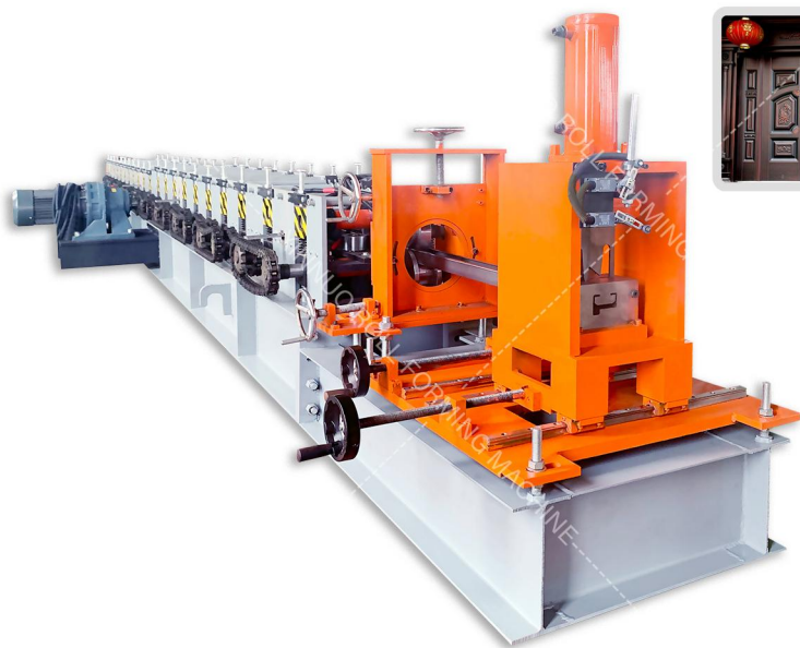
■ Garage door forming machine
