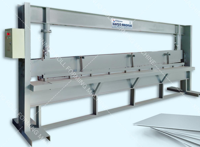
■ Hydraulic cutting machine ■ 液压剪板机
