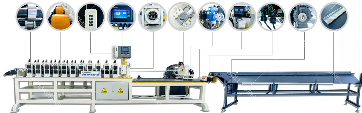
• 轻钢龙骨压型裁切主机 Profile cutting host
