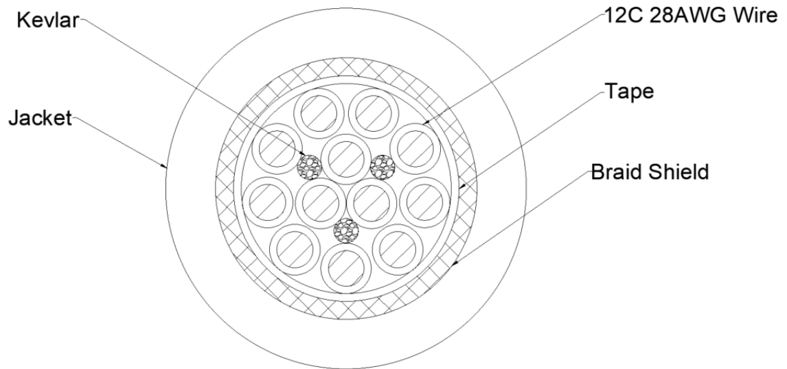
Fig.1 Cross section of cable
