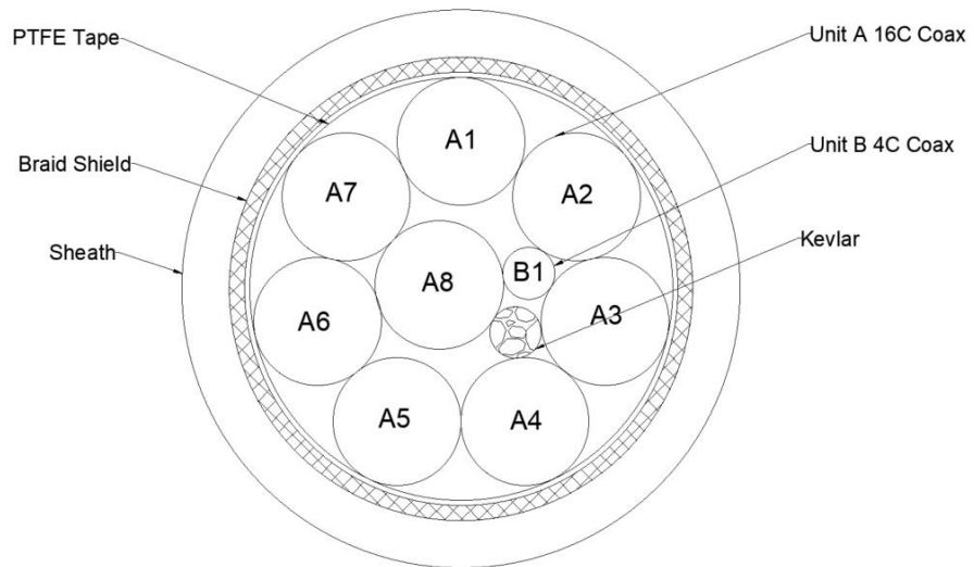
Fig.2 Cross section of cable
