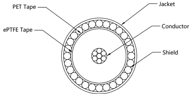
Fig.1 Cross section of 42AWG Coax
