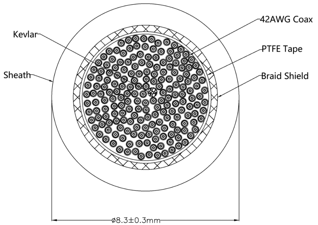
Fig.1 Cross section of cable
