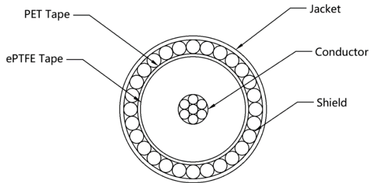
Cross section of 42AWG Coax
