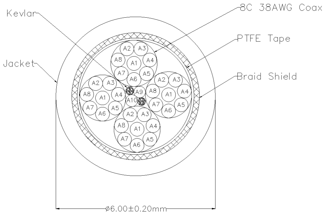
Fig.1 Cross section of cable
