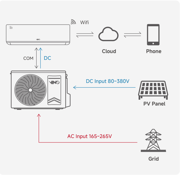
Connection 1
