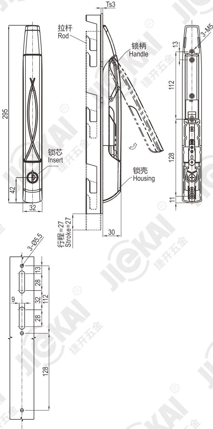
开孔尺寸 Recommended hole size
