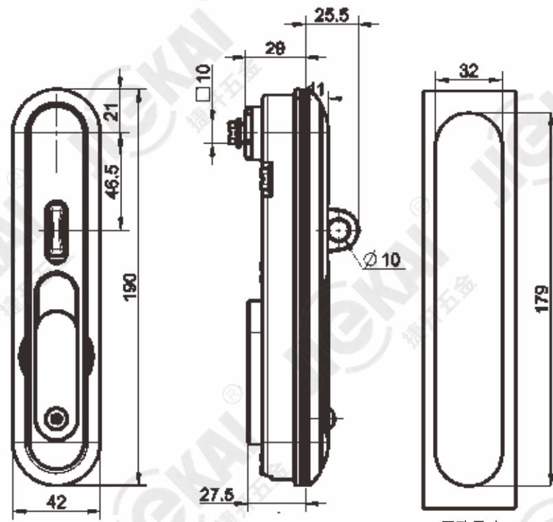
开孔尺寸 Recommended hole size
