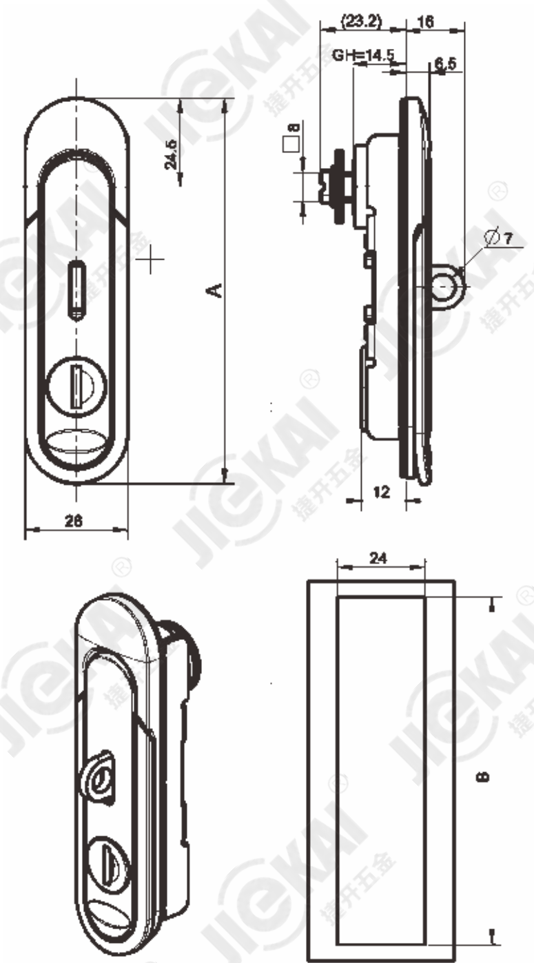
开孔尺寸 Recommended hole size
