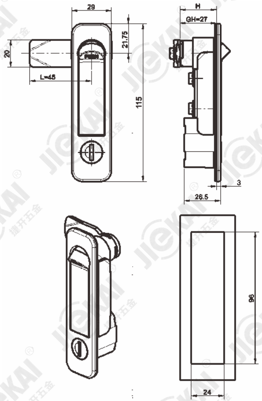
开孔尺寸 Recommended hole size
