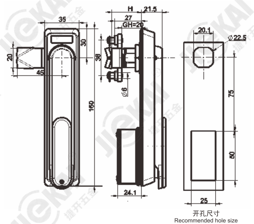
规格型号 Specifications PM212-1K3-P2
