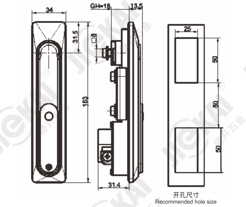
规格型号 Specifications PM211-1K3-P2
