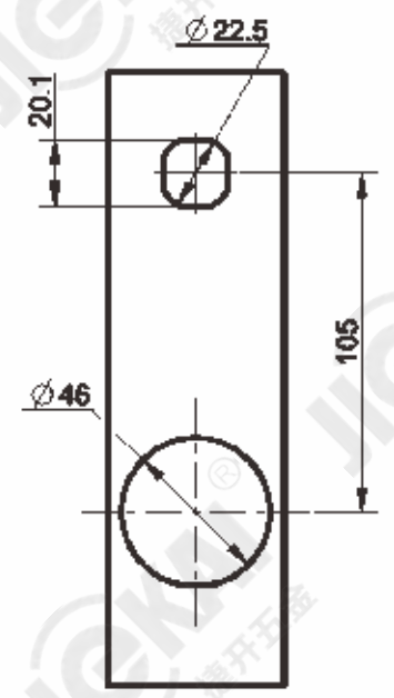
开孔尺寸 Recommended hole size
