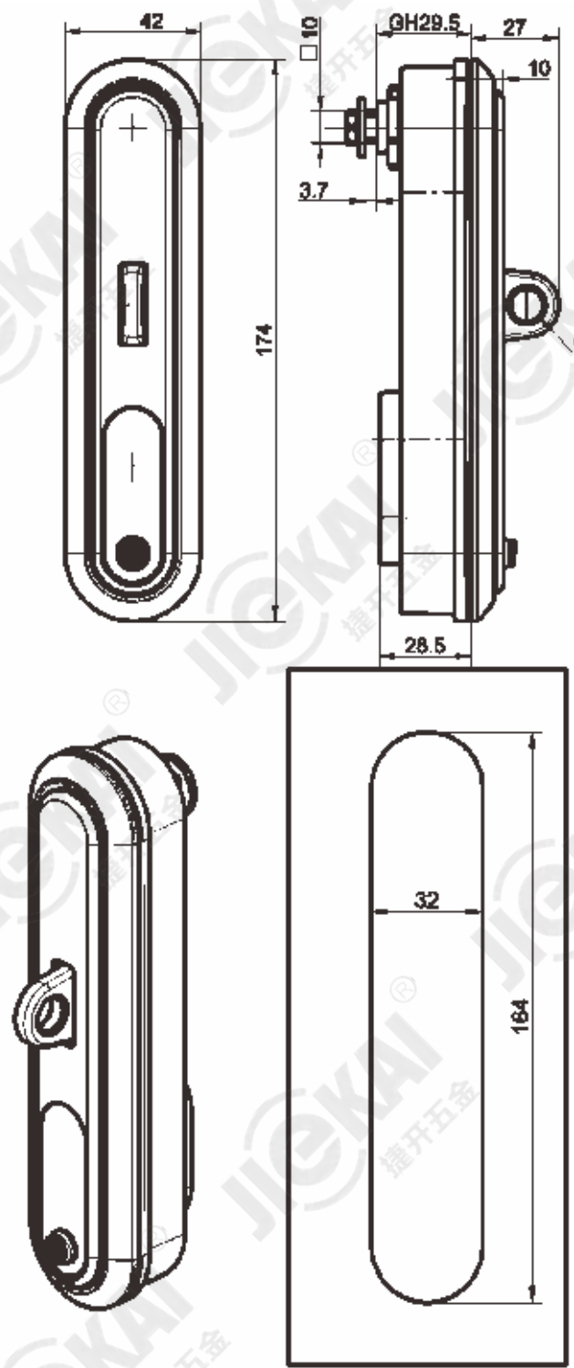
开孔尺寸 Recommended hole size
