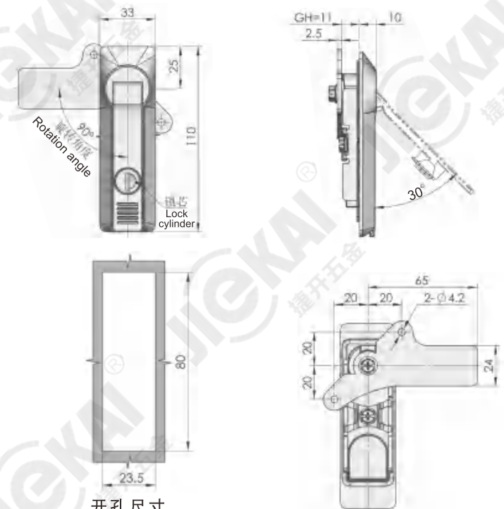
开孔尺寸 Recommended hole size
