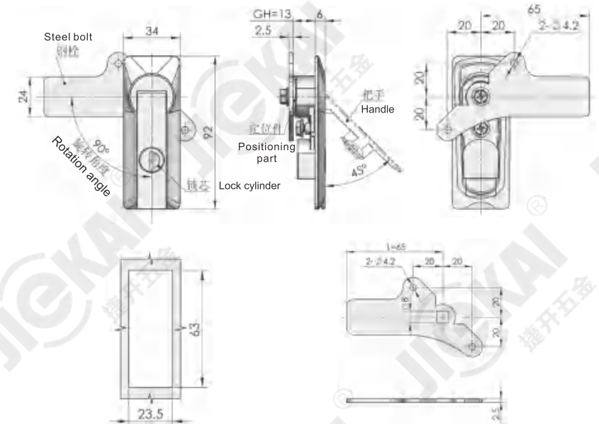
开孔尺寸 Recommended hole size
