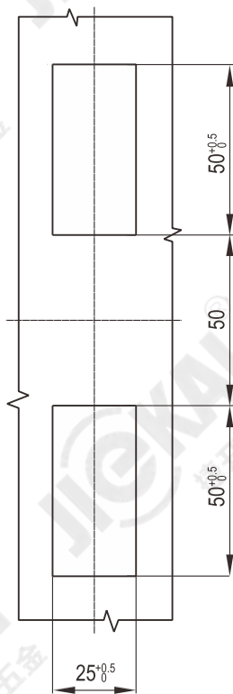
开孔尺寸 Recommended hole size
