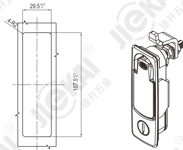
开孔尺寸 Recommended hole size
