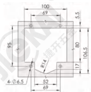
开孔尺寸 Recommended hole size
