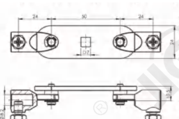
默认钢栓 Default steel bolt
