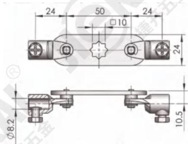
默认钢栓 Default steel bolt
