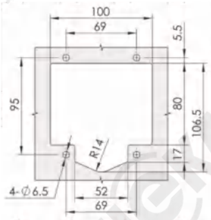
开孔尺寸 Recommended hole size
