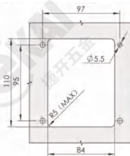
开孔尺寸 Recommended hole size
