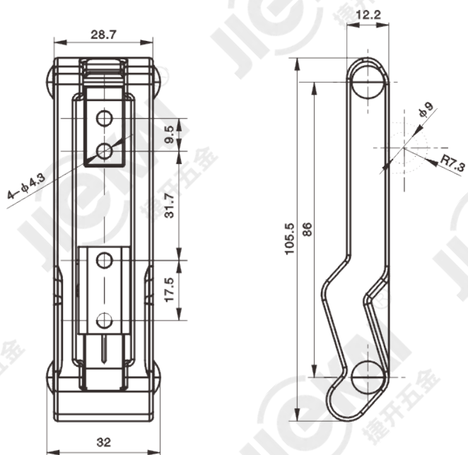
带挂 Padlockable DK937-7JXX
