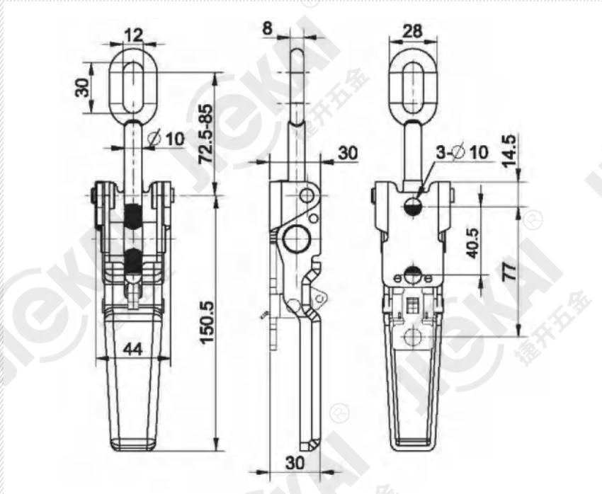
调节搭扣 Adjusting buckle DK906-6YE0
