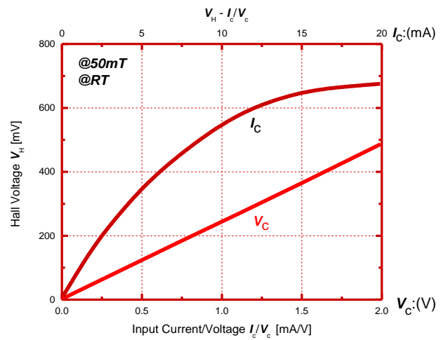
Figure 5. Hall voltage V_H as a function of electrical stimuli I_e/V_e .
