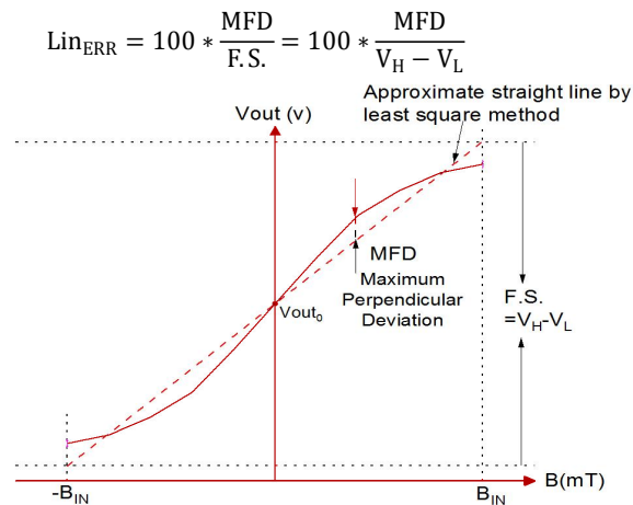
Figure 1. Output characteristics of AEG-230L
