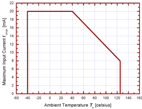
Figure 1. 2 Maximum input Current I_{cmax}
