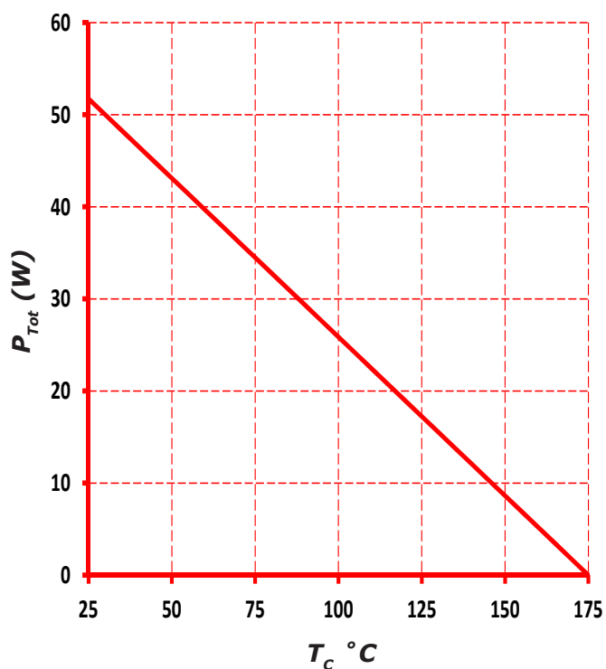
Figure 4. Power Derating
