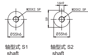
输出轴径/Output Diameter
