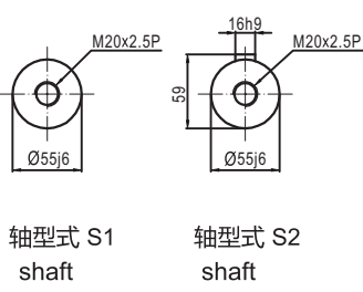
输出轴径/Output Diameter
