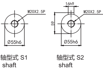
输出轴径/Output Diameter
