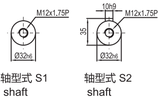
输出轴径/Output Diameter
