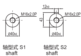
输出轴径/Output Diameter
