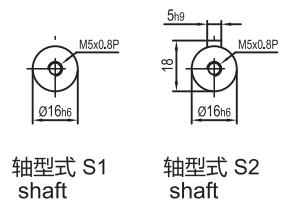
输出轴径/Output Diameter
